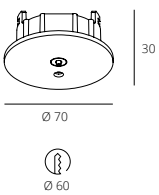
RHL77010 Recessed Box Material: Aluminum
