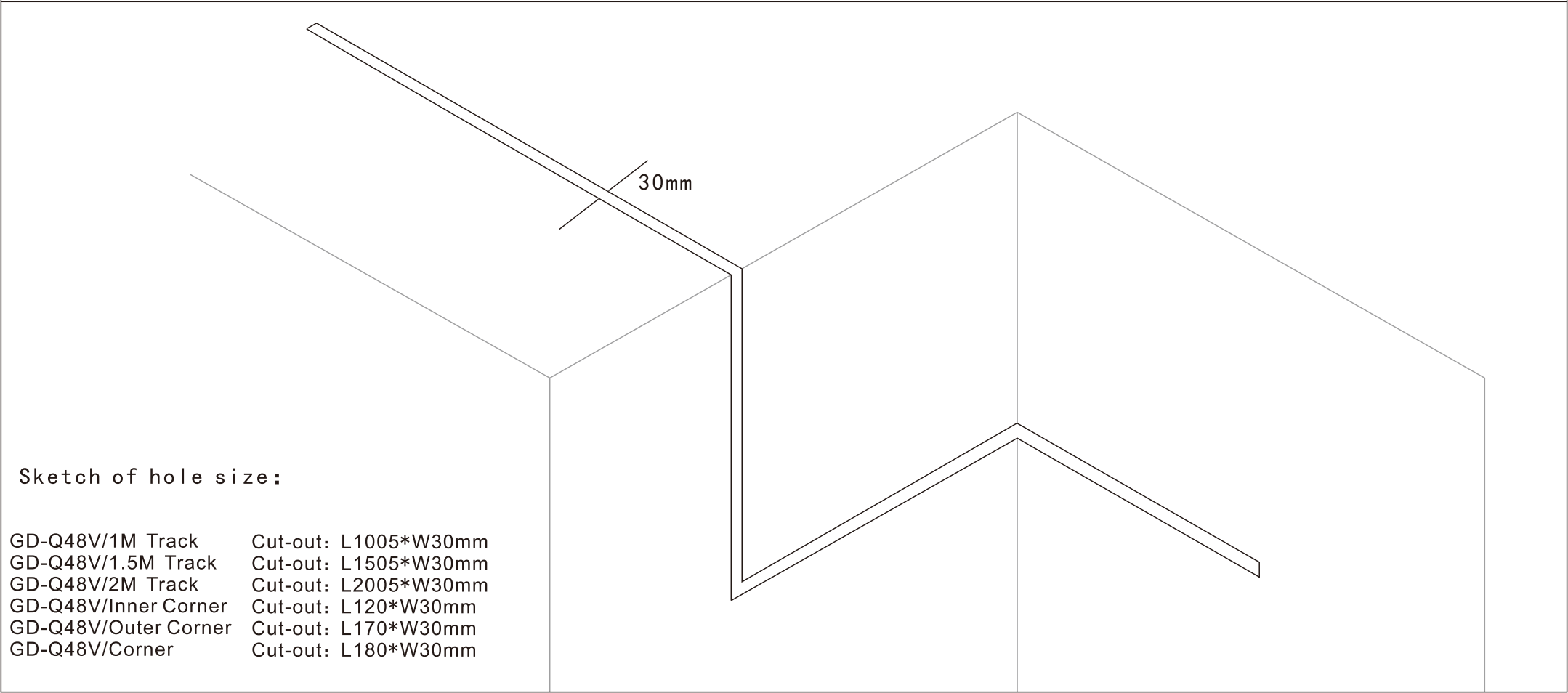
Connection diagram :
